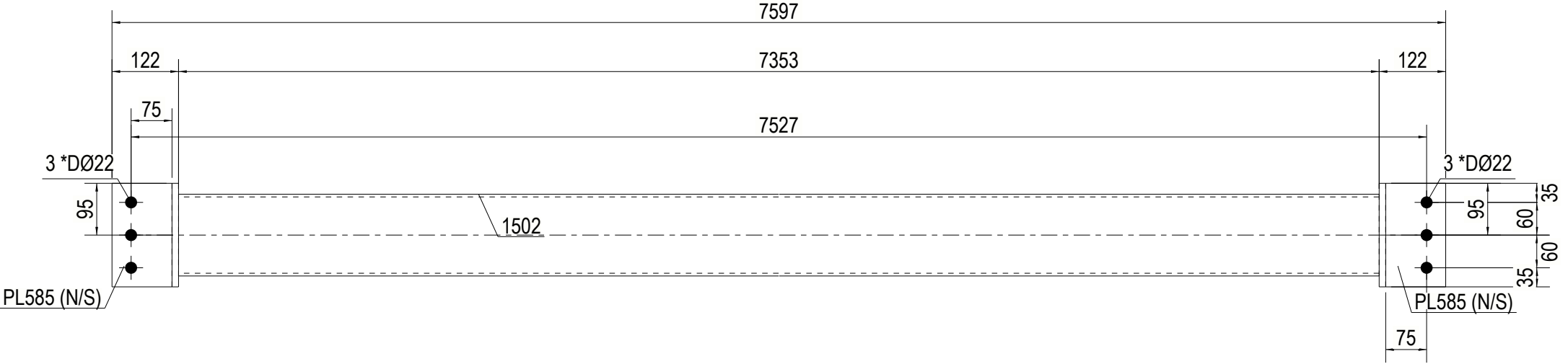
FRONT VIEW
